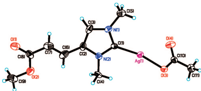
Figure 5. Crystal structure of [( 8 )AgOAc] ( 9 ). Thermal ellipsoids are shown at 50% probability.
