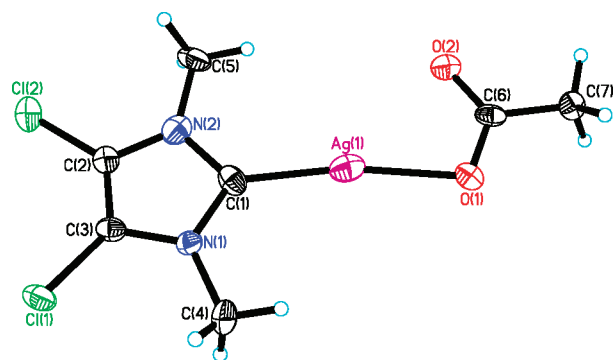
Figure 2. Crystal structure of [( 4 )AgOAc] ( 5 ). Thermal ellipsoids are shown at 50% probability.
