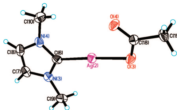
Figure 3. Crystal structure of [( 6 )AgOAc] ( 7 ). Thermal ellipsoids are shown at 50% probability.
